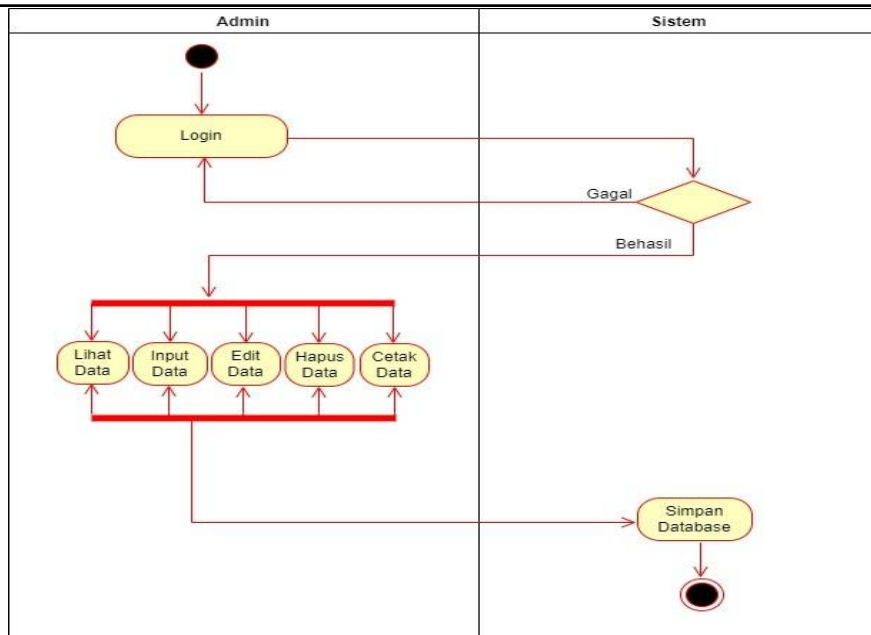
Gambar 3.2 Activity Diagram Pendataan pegawai
